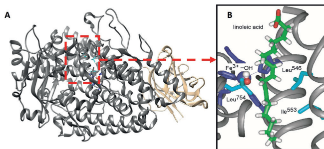
Figure 1. A) X-ray structure of SLO-1 (PDB ID: 1F8N), with active-site region highlighted by a red box and the N terminus shown in tan. B) X-ray structure of the active site of SLO-1, with LA modeled into the active site. The side chains L546, L754, and I553 are shown in cyan. Figure taken from Ref. [6b].
